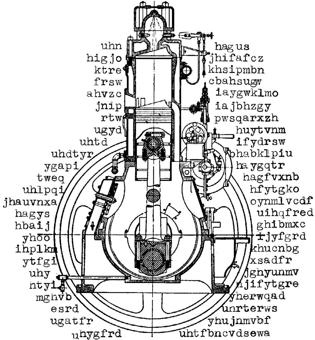
Transverse Section through Low-Compression Engine.
