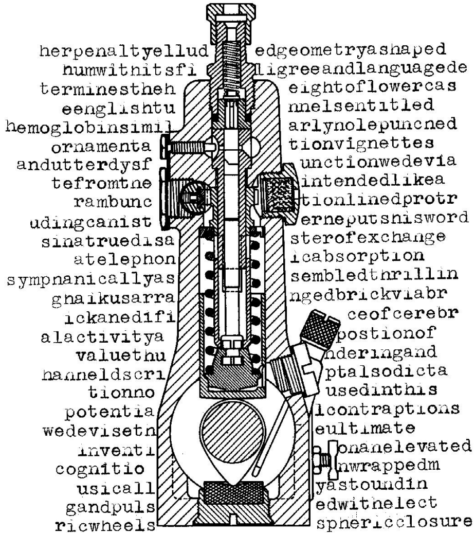
Vertical Section Thru Pump
